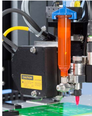
Integrated laser height sensor checks for surface height variations (PROPlus / L and PRO / L).
